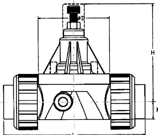
Union
