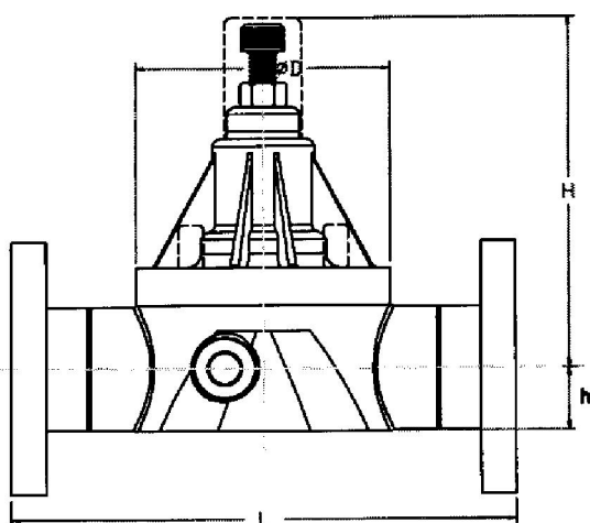
Flanged
