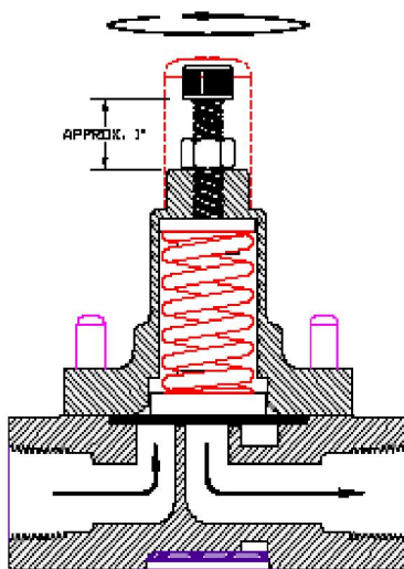
AIR RELEASE POSITION WITH HANDLE BACKED OFF
