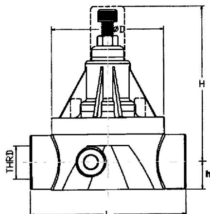
Threaded Female
