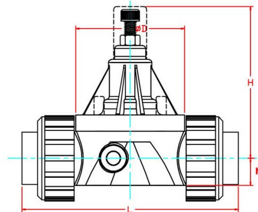
Union
