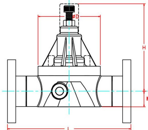
Flanged
