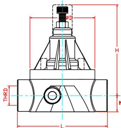
Threaded Female
