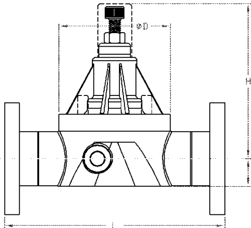
Flanged
