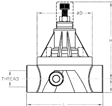
Threaded Female
